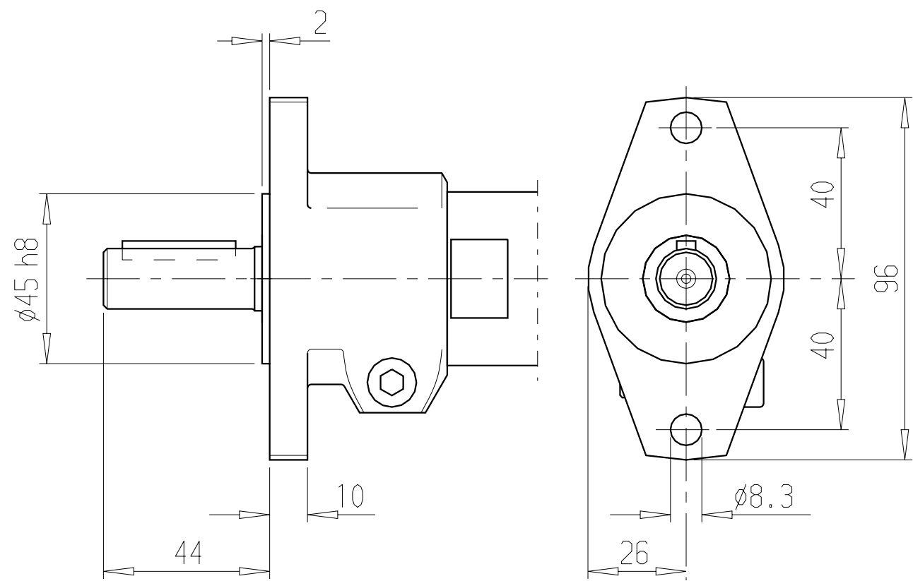
Flange Ordering No. 4430 0490 80
