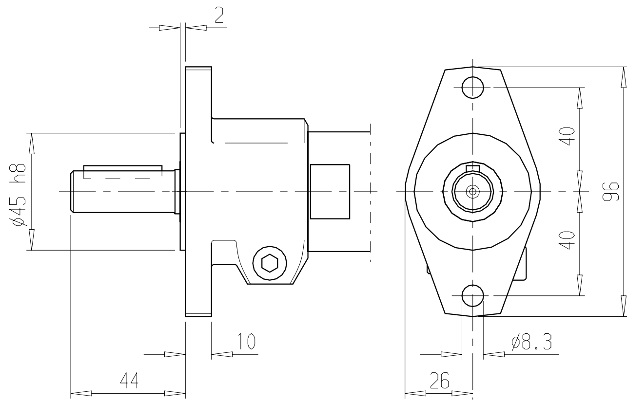
Flange Ordering No. 4430 0490 80
