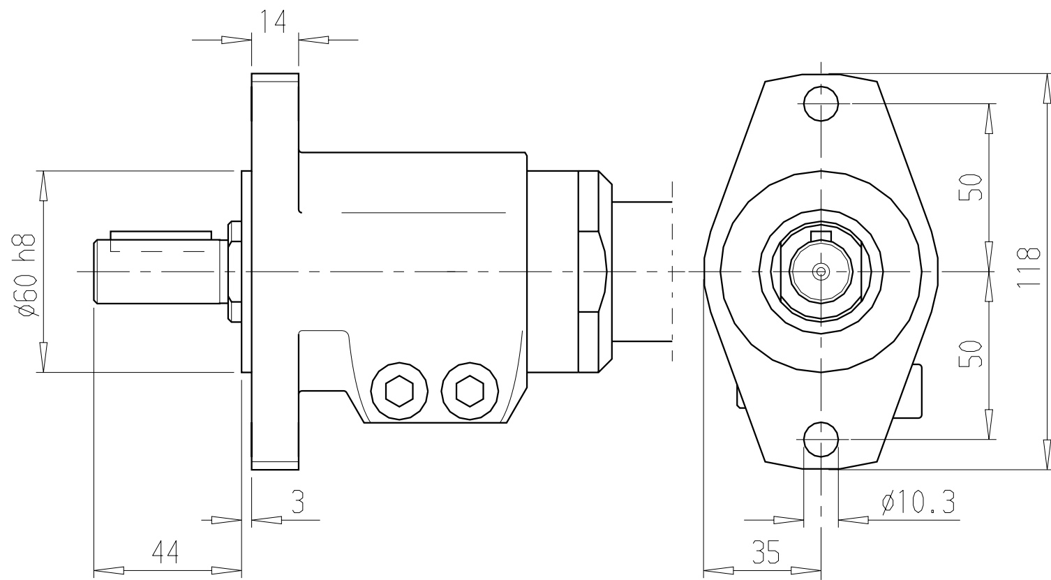
Flange Ordering No. 4430 0569 80
