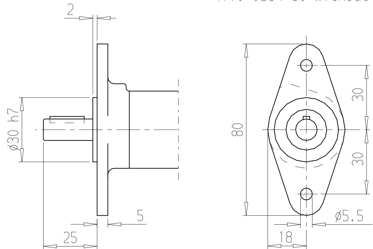
Flange Ordering No. 4110 0984 85 with holes 4110 0984 80 without holes
