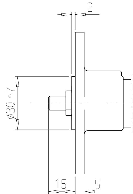
Flange Ordering No. 4430 0165 85
