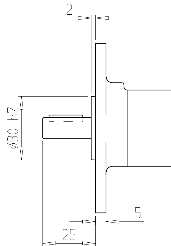
Flange Ordering No. 4110 0984 85 with holes 4110 0984 80 without holes
