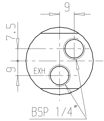
Flange Ordering No. 4110 0878 85 with holes Ordering No. 4110 0878 80 without holes
