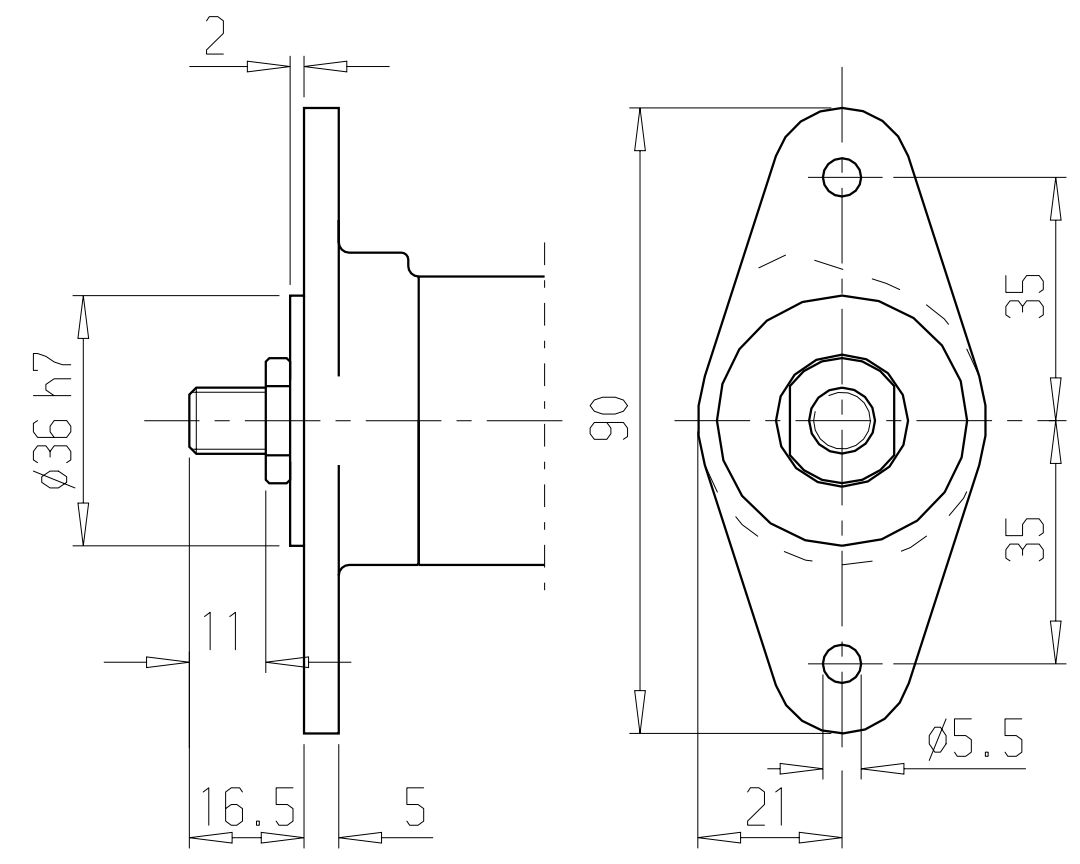
Flange Ordering No. 4110 0878 85 with holes Ordering No. 4110 0878 80 without holes
