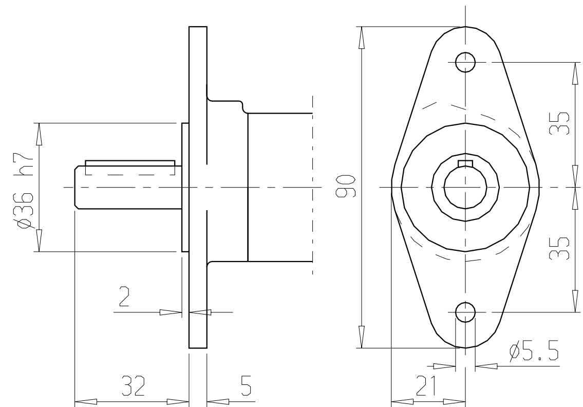
Flange Ordering No. 4110 0878 85 with holes Ordering No. 4110 0878 80 without holes
