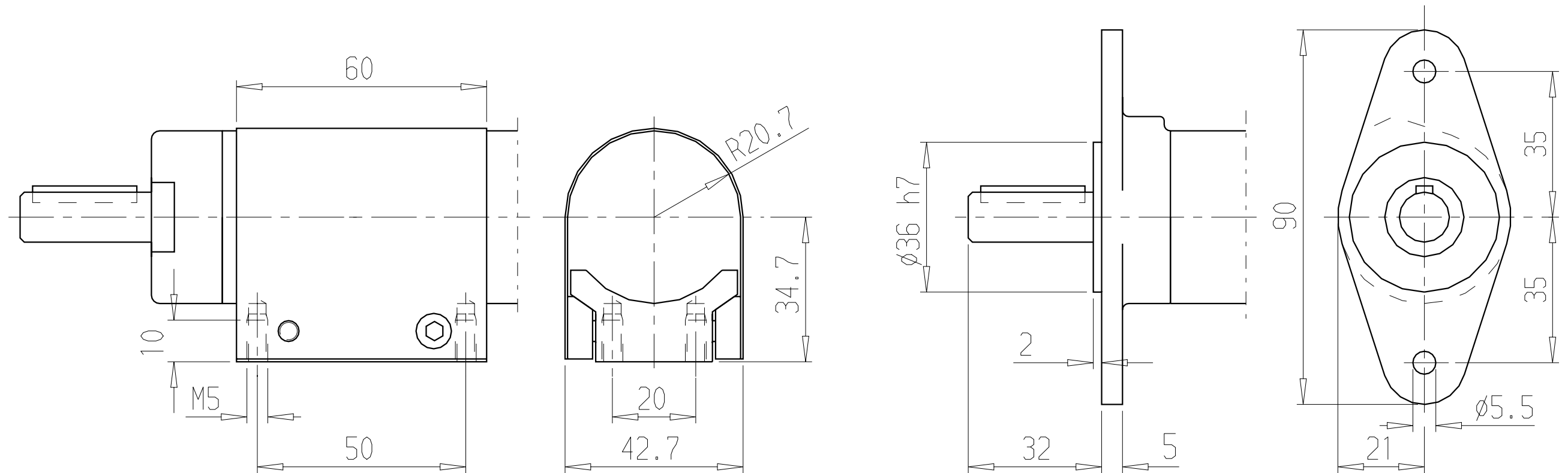
Flange Ordering No. 4110 0878 85 with holes Ordering No. 4110 0878 80 without holes
