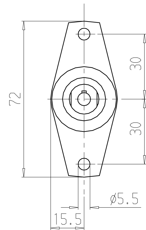
Flange Ordering No. 4430 0922 80
