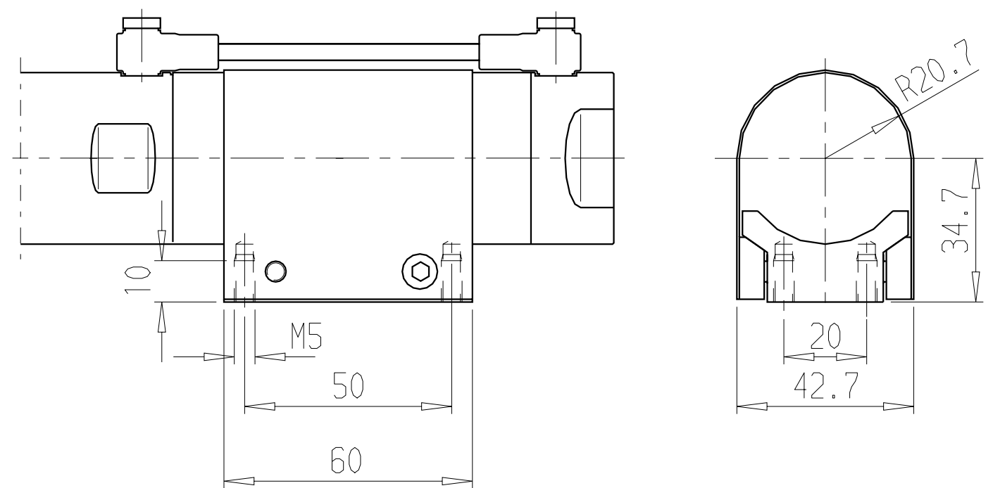
Foot Ordering No.4430 0855 80
