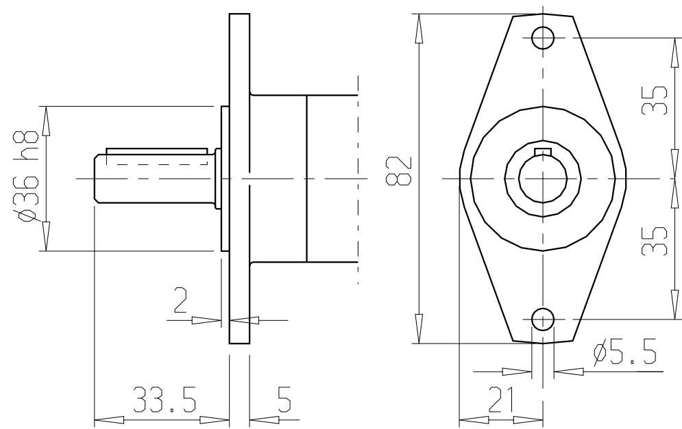
Flange Ordering No.4430 0850 80
