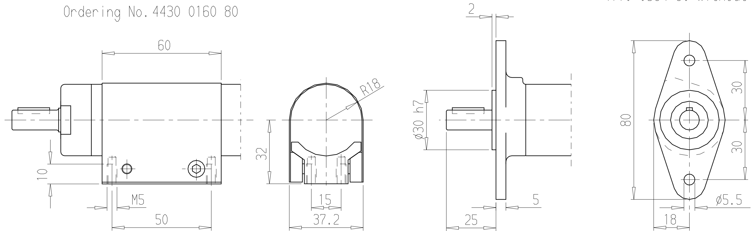
Flange Ordering No. 4110 0984 85 with holes 4110 0984 80 without holes
