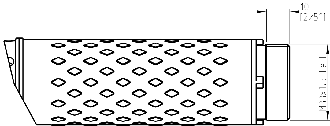
Detailed view A
